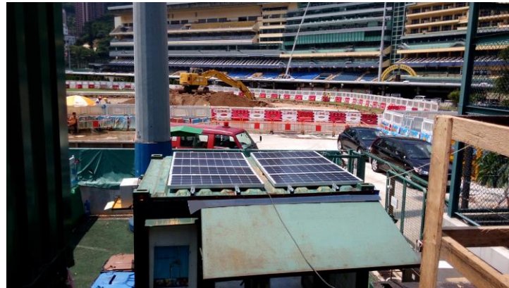
Happy Valley 0.8kW Off Grid System
